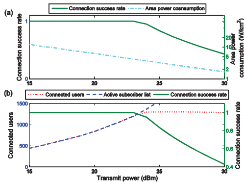
Figure 1: Transmit power for a 3-sectored base station with fixed bandwidth versus (a) connection success rate and area power consumption and (b) connected users, active subscriber list, and connection success ratio
