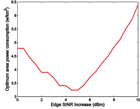
Figure 4: Optimum area power consumption calculated for different levels of edge SINR increase
