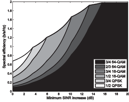
Figure 3: The relationship between spectral efficiency and increased edge SINR. Each area shows the relative contribution of that MCS to the total
