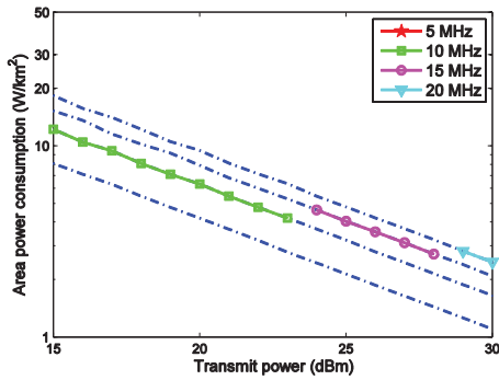
Figure 2: Area power consumption (dotted dashed lines) versus transmit power for bandwidths of 5 (lowermost line), 10, 15, and 20 MHz (uppermost line). Markers indicate the optimum area power consumption subject to constraints at each transmit power
