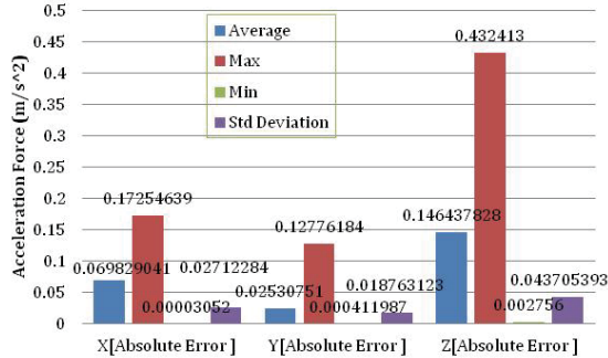
Fig. 4: Absolute Error of Accelerometer Sensor (Sampling Rate: Fastest)
