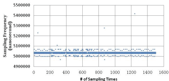
Fig. 12: Sampling frequency (Sampling Rate: Fastest)
