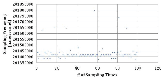
Fig. 13: Sampling frequency (Sampling Rate: Normal)
