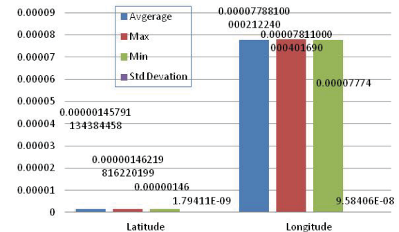
Fig. 20: Absolute Error of GPS
