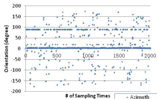
Fig. 14: The output of getOrientation() (Sampling Rate: Fastest)
