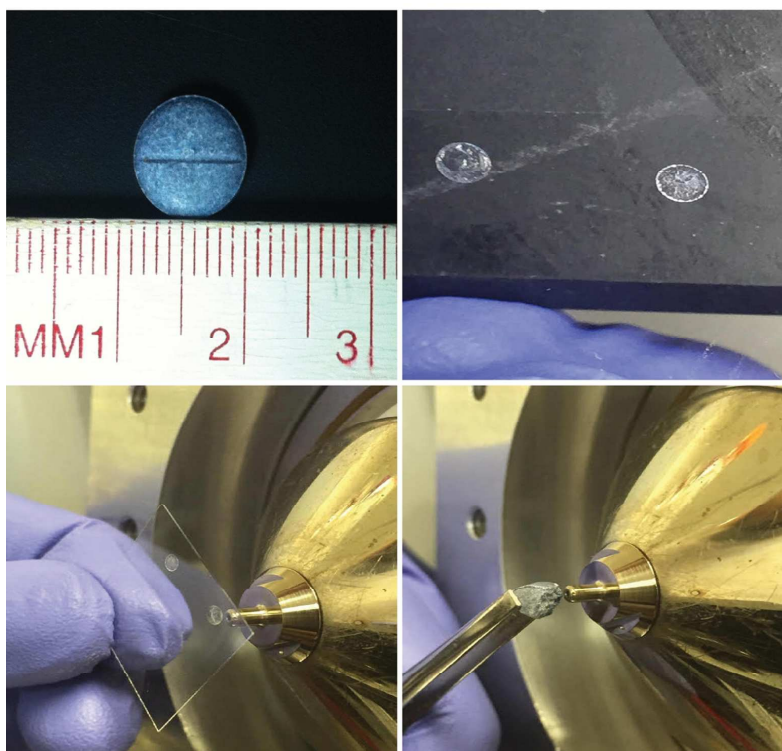
Figure 6. Top left: Tablet obtained from an UK-based vendor and sold as 2-MXP. Direct analysis was carried out by matrix assisted inlet ionization Orbitrap mass spectrometry using 3-nitrobenzotrile (3-NBN) as the matrix. Top right: mixed matrix and 2-MXP reference droplets after air-dry on glass plate. Bottom left: MAII operating with samples on cover glass. Bottom right: Direct analysis of 2-MXP tablet and confirmation of the protonated molecule by high resolution Orbitrap MS.
