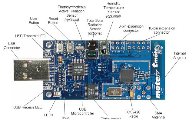
Figure 2. The front-side of T-mote Sky module.
