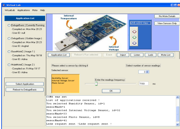
Figure 4. VLC application GUI.
