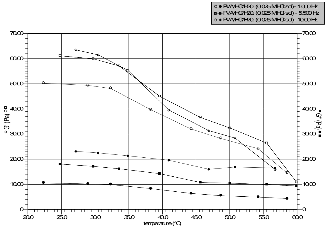
Figure 10 PVA/HCl/H 2 O (0.025M HCl solution)
