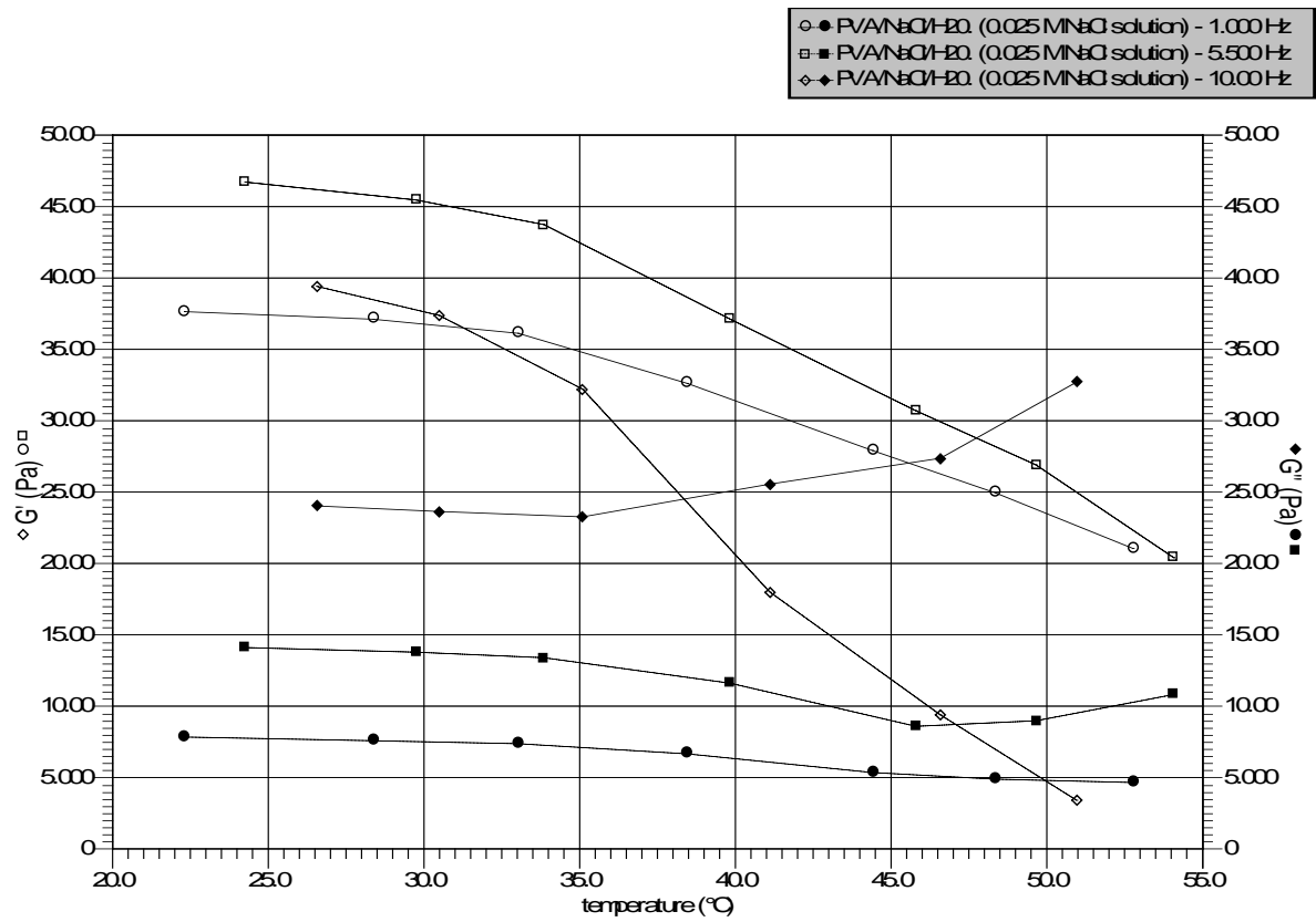
Figure 12 PVA/NaCl/H 2 O (0.025M NaCl solution)
