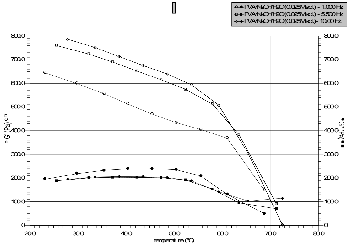
Figure 11 PVA/NaOH/H 2 O (0.025M NaOH solution)
