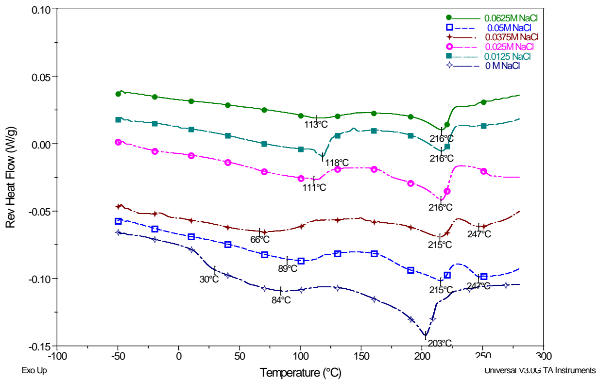
Figure 6 Reversible thermal transitions in PVA/H 2 O/NaCl
