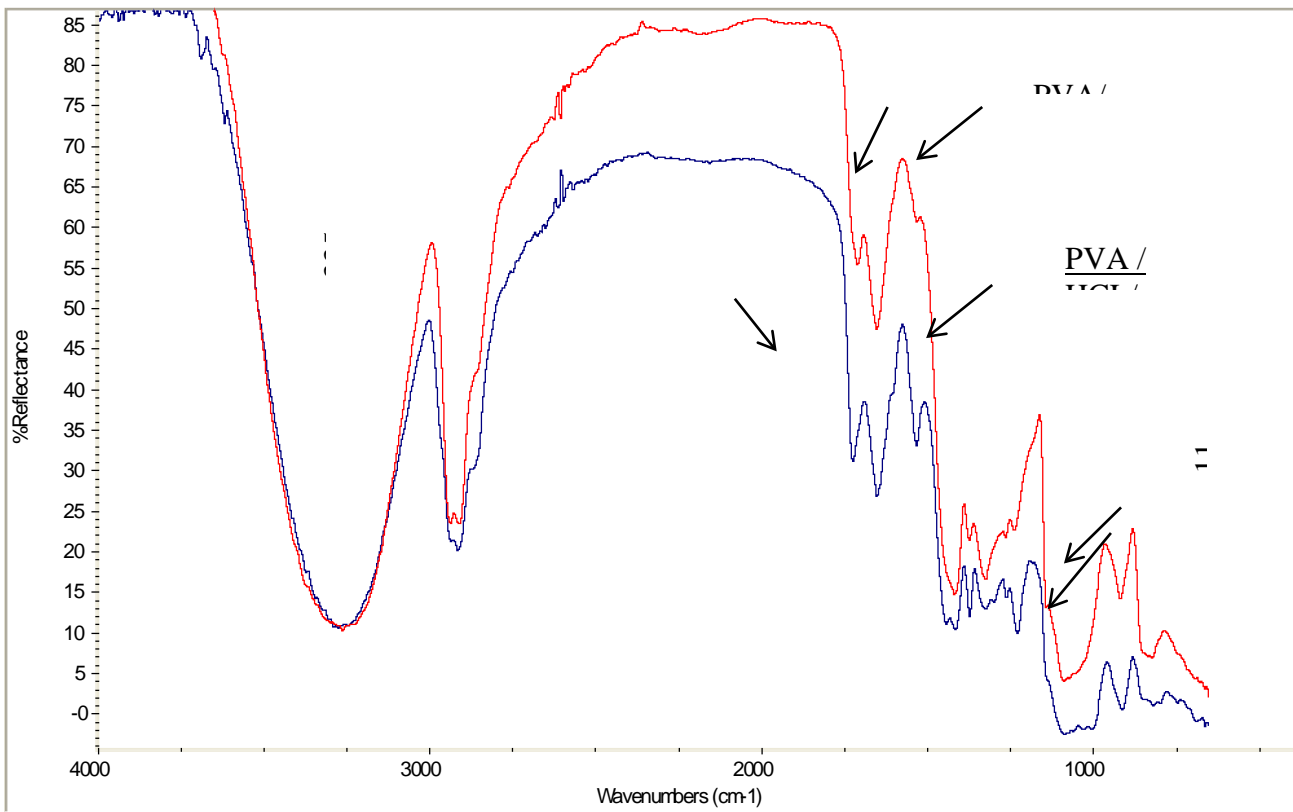
Figure 7 FTIR spectrum of pure PVA/H 2 O and, a blend of PVA/HCl/H 2 O (0.025M HCl solution)
