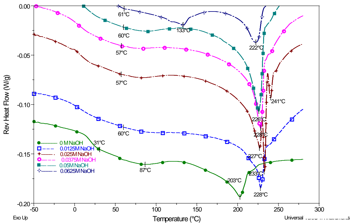
Figure 5 Reversible thermal transitions in PVA/H 2 O/NaOH
