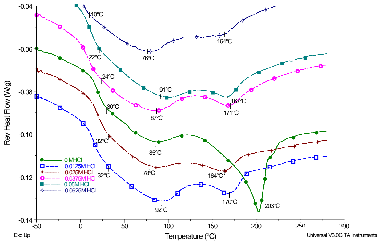
Figure 4 Reversible thermal transitions in PVA/H 2 O/HCl
