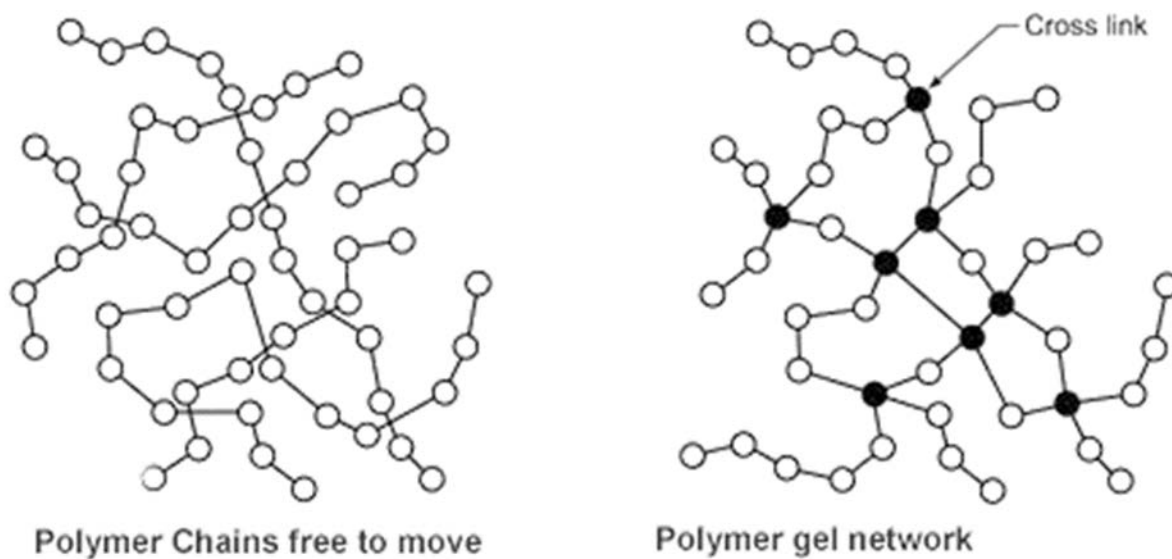
Figure 1.1 Schematic of a polymeric gel network.
