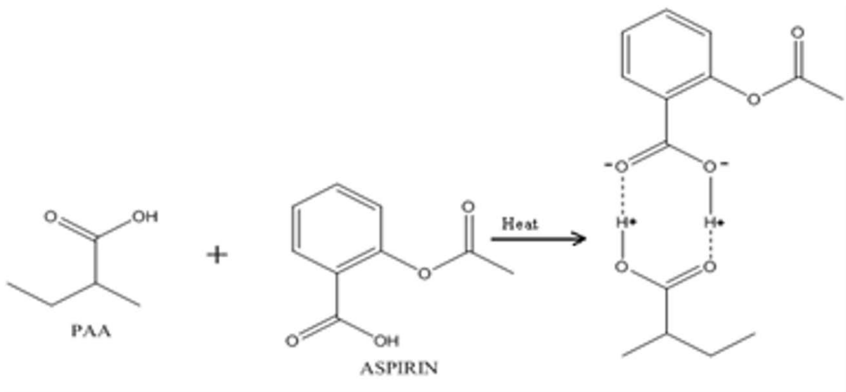
Figure 1.3 Diagram of reaction between PAA and aspirin.
