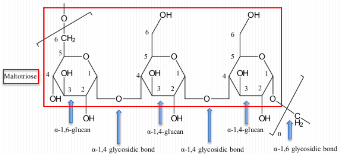
Figure 6: Chemical structure of pullulan which consist of 3 sugar repeating units.
