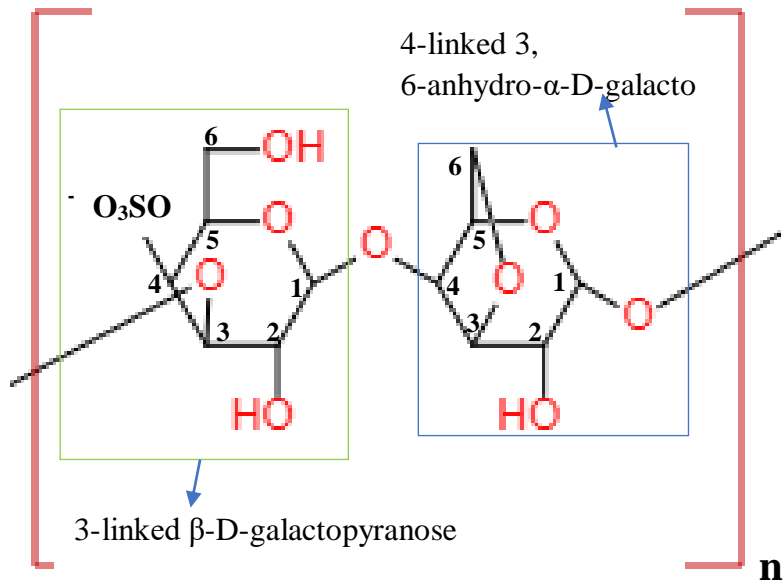
Figure 3: Chemical structure of Kappa-carrageenan.
