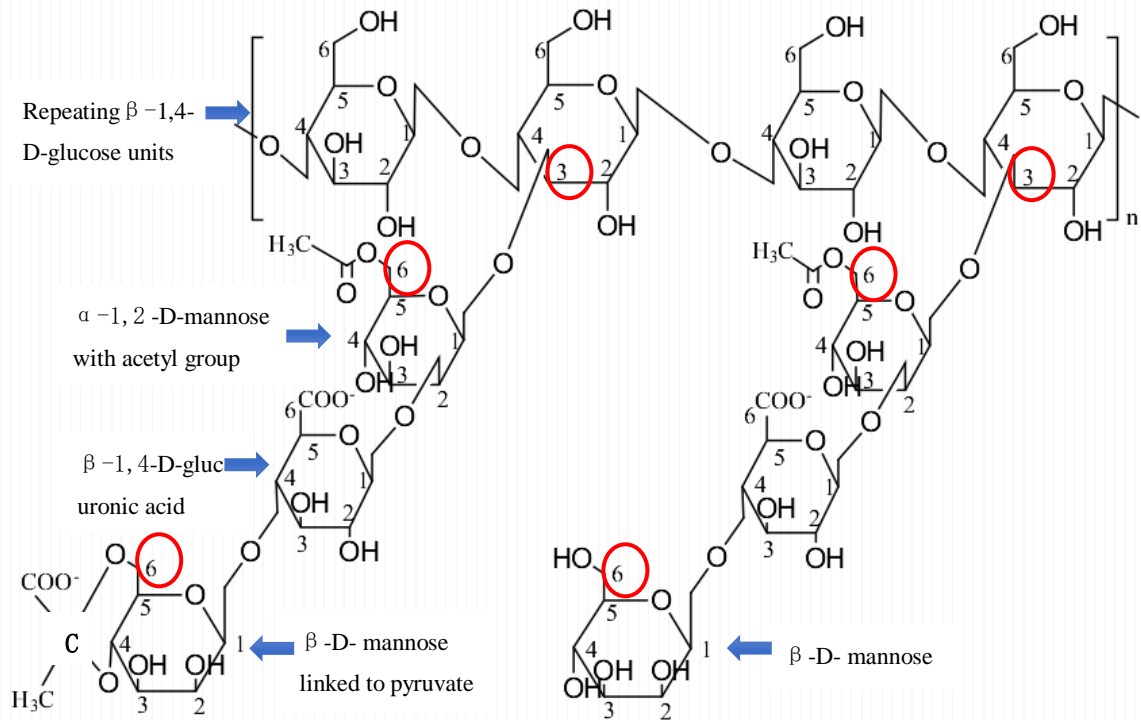
Figure 5: Chemical structure of Xantham gum which consist of 5 sugar repeating units.
