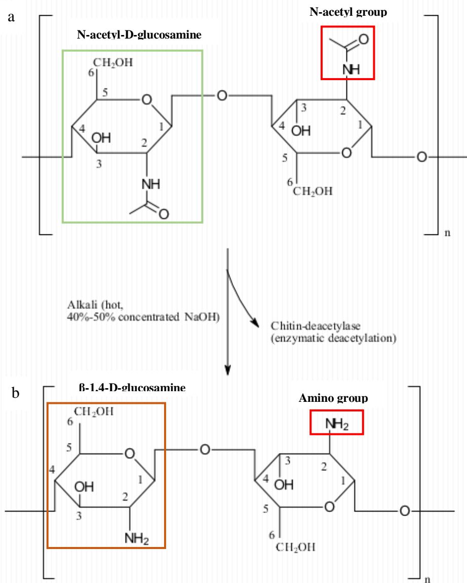
Figure 4: Chemical structure of (a) chitin and (b) chitosan.
