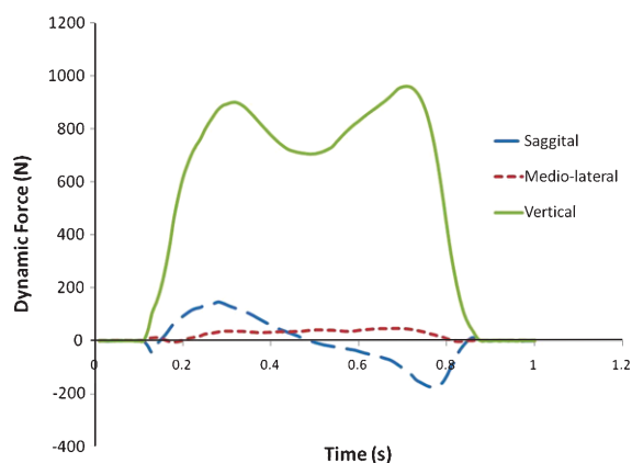
Fig. 1. Typical ground reaction force traces in three orthogonal planes.
