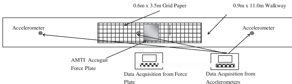
Fig. 3. Schematic representation of walkway and test set-up (not to scale).
