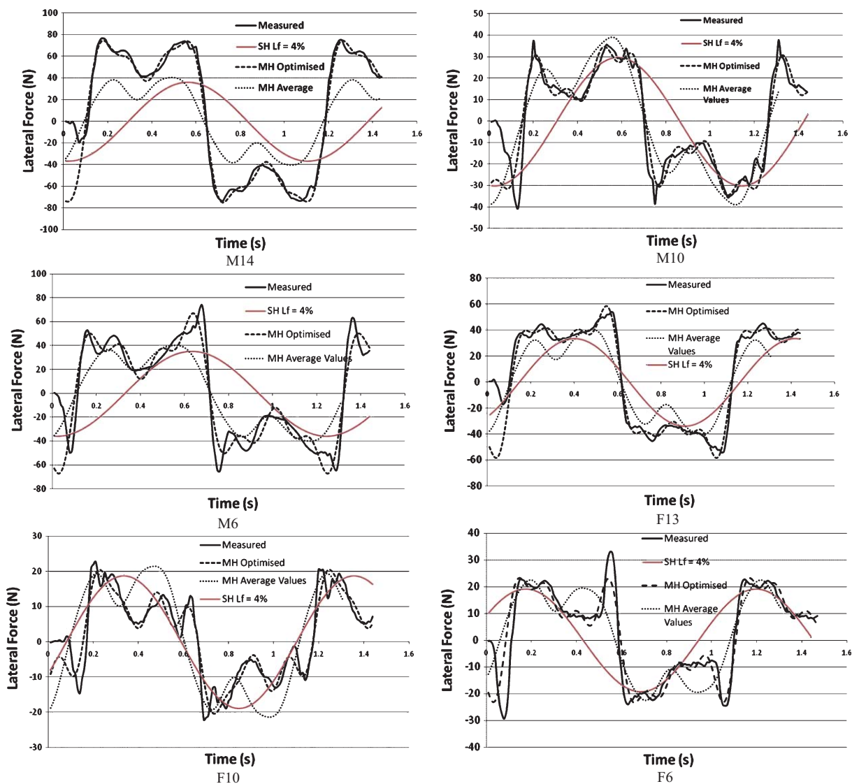
Fig. 10. Selected recorded and simulated lateral force functions.
