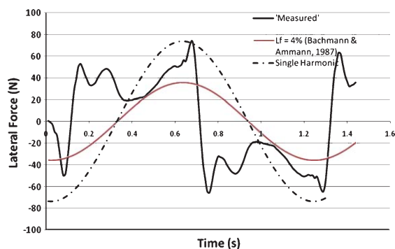
Fig. 9. Lateral force recorded and simulated using single harmonic load function for M12.
