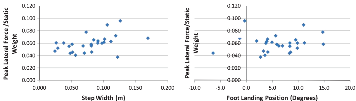
Fig. 7. Relationship of peak lateral force/static weight to step width and foot landing position respectively.
