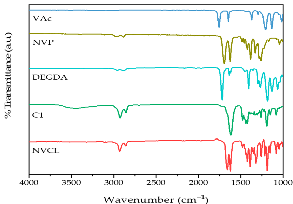
Figure 3. FTIR spectra of (top–bottom) VAc monomer, NVP monomer, DEGDA monomer, PVNCL100, and NVCL neat.
