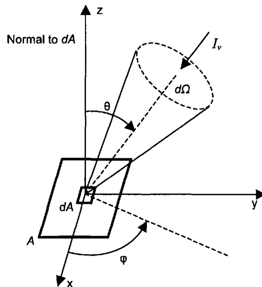
Figure 3.17 Basic geometry for radiation of intensity I_\nu incident on a flat area
