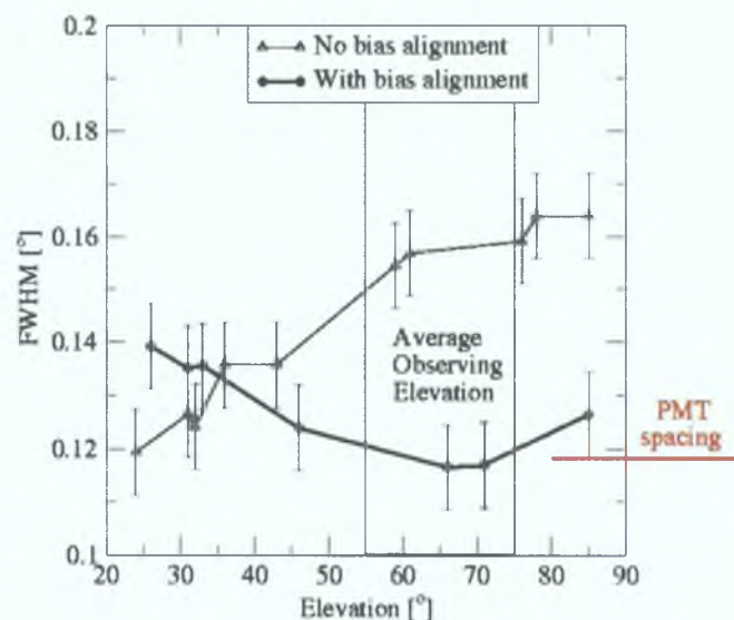
Figure 3.10 PSF measurements for the Whipple 10m reflector. The spacing of the PMTs in the imaging camera of the telescope is also indicated. Figure from Kildea et al (2007).
