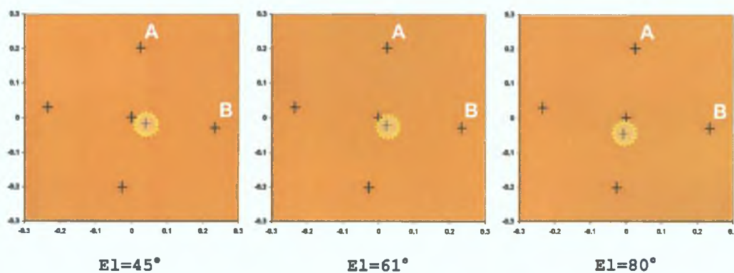
Figure 4.11 Simulated star images at the focal plane.
