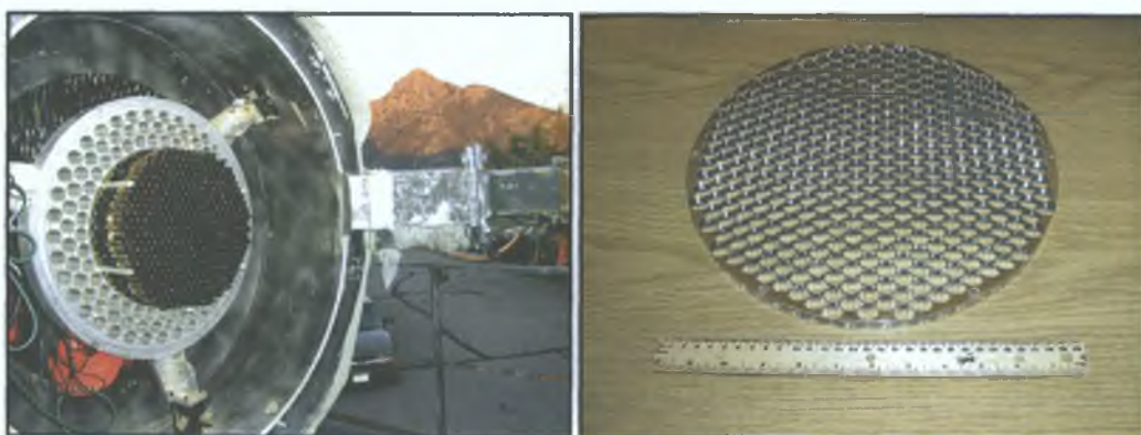
Figure 3.5 Left: The 379-PMT camera (without lightcones) in the focus box of the telescope. On the picture is partially visible one of the four arms, and Mount Wrightson in the background. Right: The lightcone plate, which fits onto the front of the camera.
