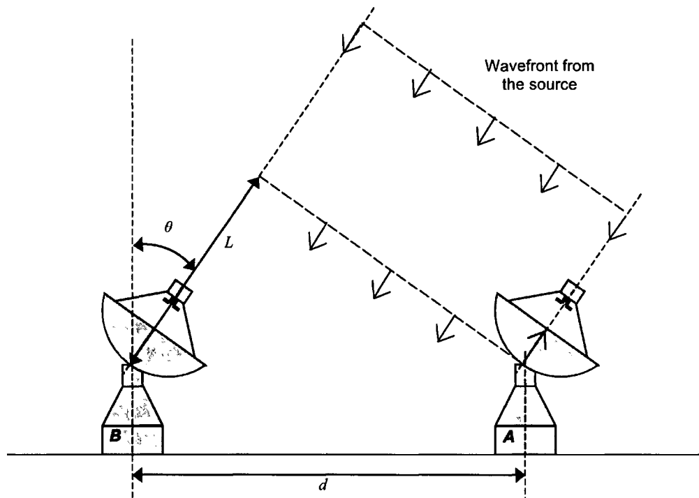
Figure 3.19 Radio interferometry
