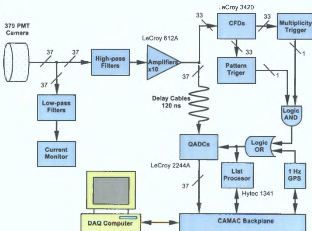
Figure 3.11 Data Acquisition System.
