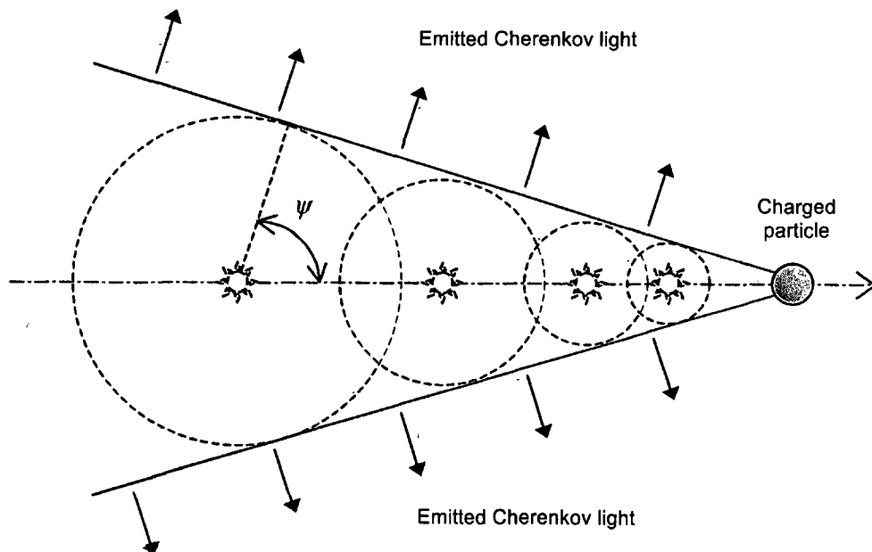
Figure 2.3 Cherenkov radiation from a moving charged particle.
