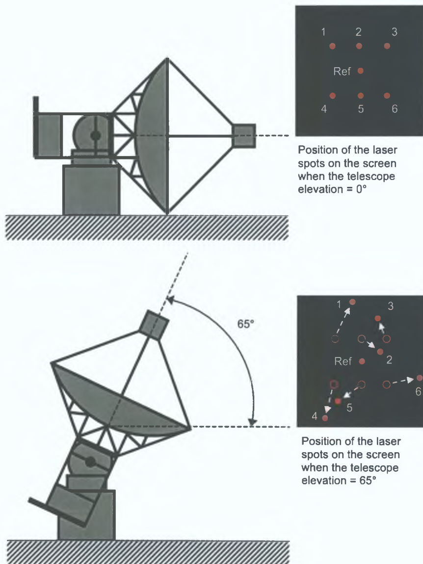
Figure 3.7 Bias measurements procedure.
