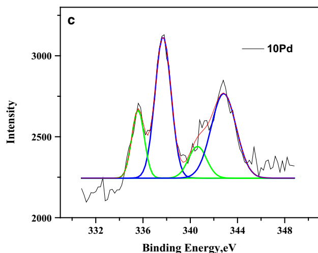
Fig. 5 XPS spectra of Pd doped titania nanotube samples a Ti 2p, b O1s, c Pd 3d of 10 Pd sample
